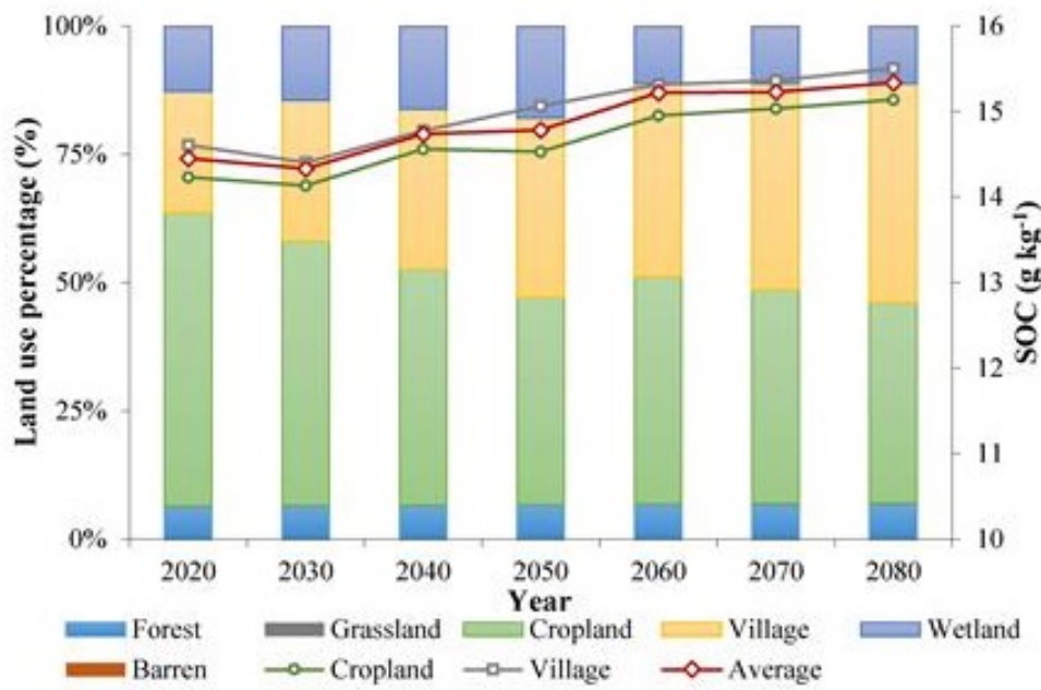
Soil organic carbon concentration ( \text{g kg}^{-1} ) dynamics concerning land use change in the study area for 2020-2080.
