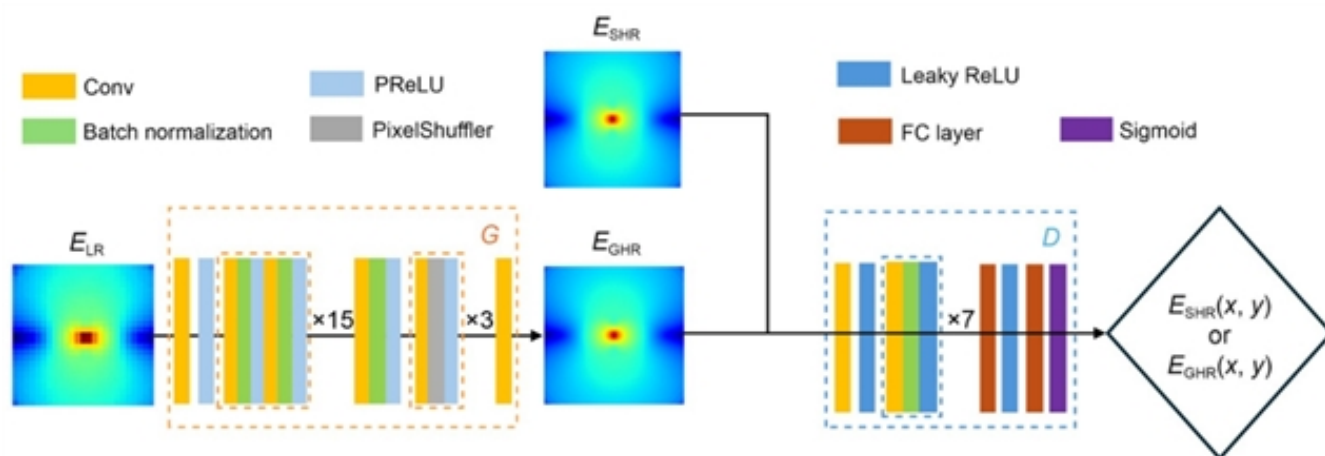
Fig. 1 Framework of EFGraGAN
