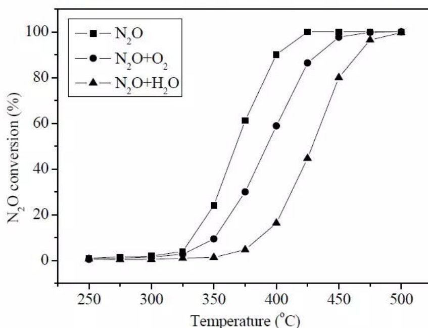
Fig. S4 N_2O conversion on CZ-1 as a function of reaction temperature, either in the absence or in the presence of 5% O_2 or 2% H_2O .
